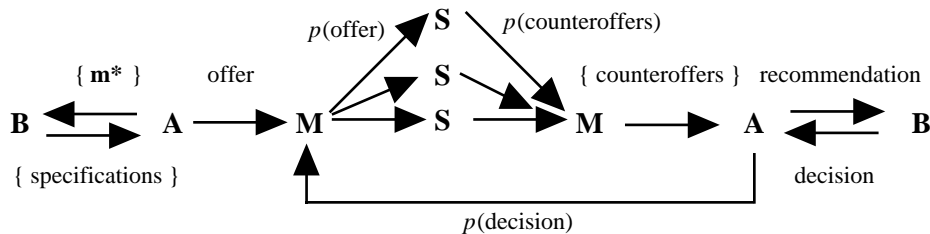
Figure 2. Schematic representation of the negotiation problem P
